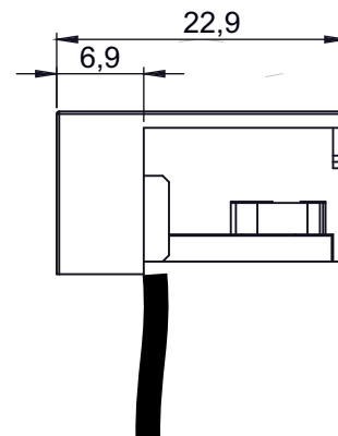
END CUP
