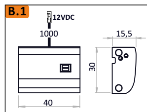
Movement 10.01.125.XY/MOV
