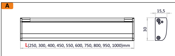
Profil Set 10.01.125.XY/Lmm
