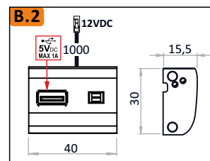
Movement+USB 10.01.125.XY/MOV/USB
