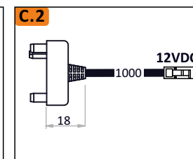
Connector 6 Right with cable 10.01.125.XY/CON6
